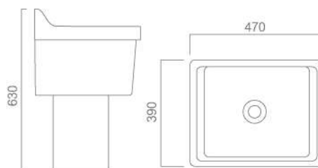
TA-011 Mop sink Size: 470x390x630mm
